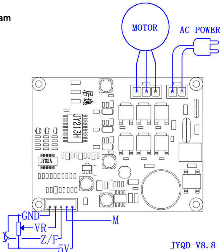
Driver board diagram
